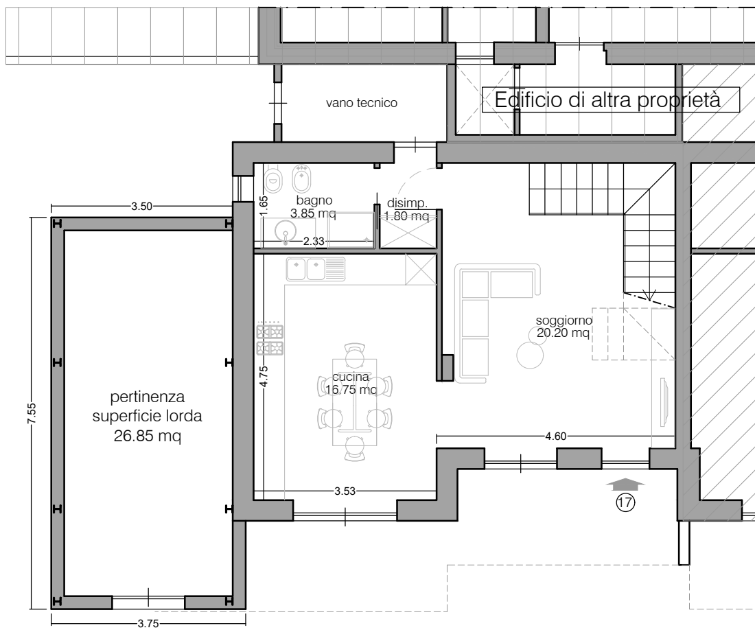
PIANO TERRA scala 1:100
